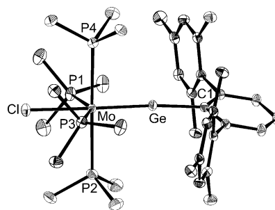
Figure 3. ORTEP plot of the structure of the complex cation of 2-Mo in the solid state. The thermal ellipsoids are set at 30% probability. Hydrogen atoms are omitted for clarity. Selected bond lengths [Å] and angles [°] of 2-Mo (bond angles and lengths of 2-W are given in square brackets): M–Ge 2.3023(4) [2.321(2)], M–Cl 2.4878(9) [2.499(4)], M–P1 2.537(1) [2.531(4)], M–P2 2.539(1) [2.526(4)], M–P3 2.532(1) [2.518(4)], M–P4 2.536(1) [2.523(4)], Ge–C1 1.962(3) [1.931(15)]; M–Ge–C1 175.3(1) [172.9(4)], Ge–M–Cl 177.75(3) [175.7(1)], Ge–M–P1 101.82(3) [101.4(1)], Ge–M–P2 91.12(3) [92.9(1)], Ge–M–P3 105.01(3) [106.9(1)], Ge–M–P4 87.76(3) [87.1(1)], Cl–M–P1 76.13(3) [75.1(1)], Cl–M–P2 89.81(3) [89.5(2)], Cl–M–P3 77.02(3) [76.6(1)], Cl–M–P4 91.35(3) [90.6(1)].
